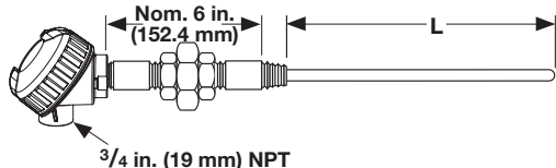
Type 1 - 6 inch N-U-N typical (2 each 1/2 x 3 inch steel pipe nipples and 1 each malleable union)
